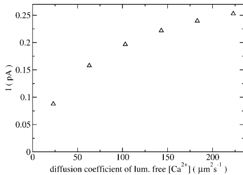
FIGURE 9 Dependence of the release current with four open channels at t = 0.1 s on the diffusion coefficient of luminal free \text{Ca}^{2+} . D_E, h_{ER} = 0.028 \mu\text{m} , concentration of free \text{Ca}^{2+} in the ER 715 \mu\text{M} , total luminal concentration 67.87 mM, B_{Em} = 0 , B_{Es} = 100 mM. For other parameter values see Set 1 of Table 1.
