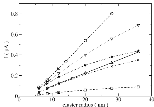
FIGURE 4 Dependence of current on cluster radius at t = 0.1 s. ( \Delta ) Set 1 except h_{\text{ER}} = 0.06 \mu\text{m} , D_E = 23 \mu\text{m}^2 \text{s}^{-1} , D_{\text{Em}} = 3.1 \mu\text{m}^2 \text{s}^{-1} . ( \circ ) Set 1, except B_{\text{Es}} = 100 \text{ mM} , B_{\text{Em}} = 0 , ( \times ) Set 1 except E = 336 \mu\text{M} , total luminal content 5.24 mM, B_{\text{Es}} = 100 \text{ mM} , B_{\text{Em}} = 0 . ( \nabla ) Set 1 except total luminal content 7.43 mM, h_{\text{ER}} = 0.06 \mu\text{m} , D_E = 110 \mu\text{m}^2 \text{s}^{-1} , D_{\text{Em}} = 16.95 \mu\text{m}^2 \text{s}^{-1} , B_{\text{Es}} = 100 \text{ mM} , B_{\text{Em}} = 0 . ( \square ) Set 1 except E = 127.8 \mu\text{M} , total luminal content 2.80 mM, B_{\text{Es}} = 100 \text{ mM} , B_{\text{Em}} = 0 . ( * ) Set 1 except E = 715 \mu\text{M} , total luminal content 7.43 mM, B_{\text{Es}} = 100 \text{ mM} , B_{\text{Em}} = 0 .
