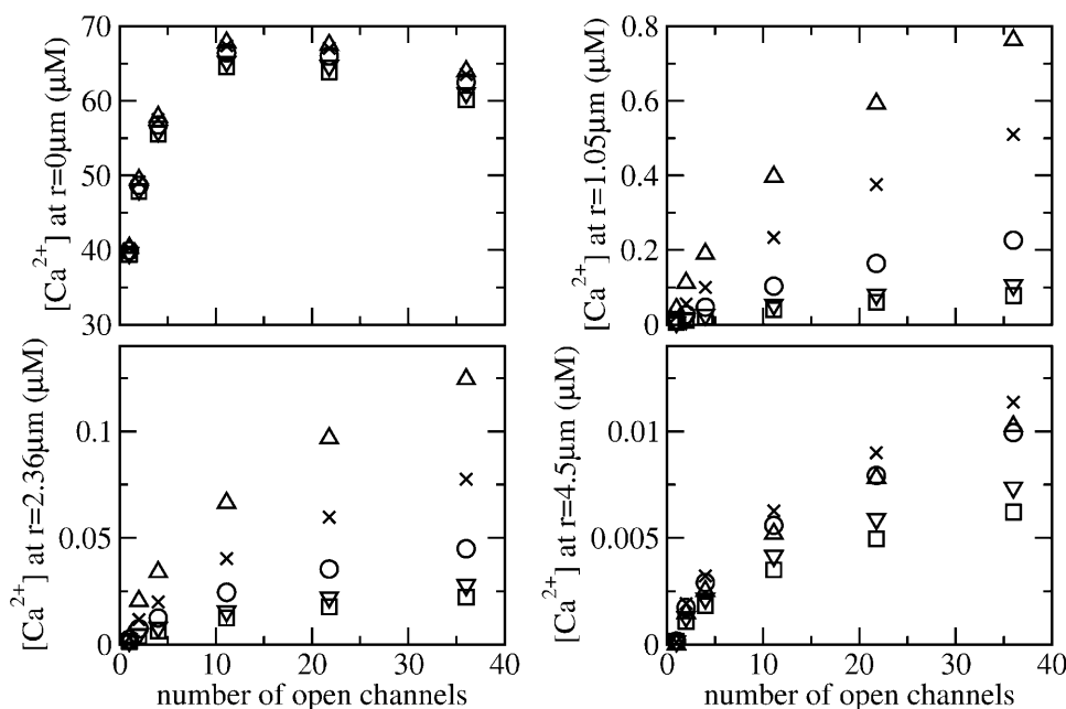
FIGURE 12 \text{Ca}^{2+} concentration at different distances from the cluster for different concentrations of mobile buffer. B_{\text{m}} = 0 \mu\text{M} ( \Delta ), B_{\text{m}} = 5 \mu\text{M} ( \times ), B_{\text{m}} = 15 \mu\text{M} ( \circ ), B_{\text{m}} = 30 \mu\text{M} ( \nabla ), B_{\text{m}} = 40 \mu\text{M} ( \square ) all k_{\text{m}}^+ = 700 ( \mu\text{Ms}^{-1} ), K_{\text{m}} = 0.247 \mu\text{M} , and D_{\text{m}} = 40 \mu\text{m}^2 \text{s}^{-1} . The currents at 0.4 s belonging to the numbers of open channels for which data are shown are: 0.041 pA (at 0.115 s), 0.071 pA, 0.119 pA, 0.218 pA, 0.299 pA, and 0.366 pA. For parameter values, see Set 1 in Table 1 except the total concentration of \text{Ca}^{2+} in the ER. It is 49 mM resulting in a resting concentration of free \text{Ca}^{2+} in the ER of 336.7 \mu\text{M} , B_{\text{Es}} = 100 mM, and B_{\text{Em}} = 0 .
