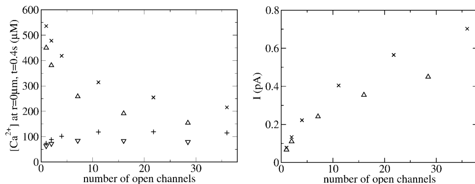
FIGURE 8 Release with parameters mimicking a tubular ER. (Left panel) Concentration of free \text{Ca}^{2+} at the cluster in dependence on the number of open channels. (X and +) Set 2 in Table 1, luminal concentration (X), cytosolic concentration (+); ( \triangle and \nabla ) Set 2 in Table 1 except D_{\text{E}} = 63\mu\text{m}^2\text{s}^{-1} , D_{\text{Em}} = 8.475\mu\text{m}^2\text{s}^{-1} , luminal concentration ( \triangle ), cytosolic concentration ( \nabla ). (Right panel) Currents for the same parameters as used in the simulations of the left panel. The symbols are chosen accordingly.
