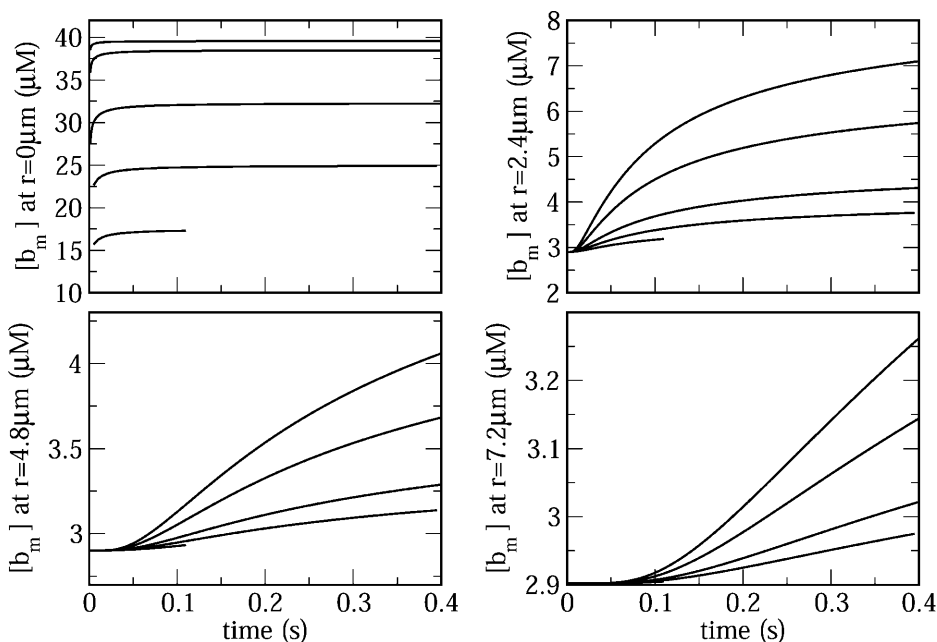
FIGURE 6 Dependence of concentration of cytosolic mobile buffer with \text{Ca}^{2+} bound on time belonging to the simulations shown in Fig. 5. The lines show results for 1, 2, 4, 11.11, and 21.77 open channels from lower to higher values. For parameter values, see Set 1 in Table 1. Release through a single channel was simulated for 0.115 s only.
