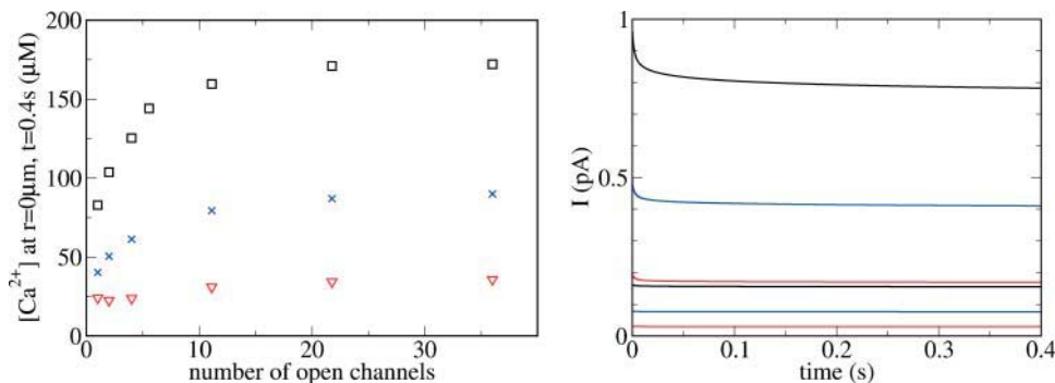
FIGURE 10 Release with different initial concentrations of free luminal \text{Ca}^{2+} . (Left panel) \text{Ca}^{2+} concentration at the location of the cluster: E = 715.56 \mu\text{M} ( \square ), total concentration of \text{Ca}^{2+} in the ER 67.87 mM; E = 336.59 \mu\text{M} ( \times ), total concentration of \text{Ca}^{2+} in the ER 49.36 mM; and E = 127.80 \mu\text{M} ( \nabla ), total concentration of \text{Ca}^{2+} in the ER 26.87 mM. (Right panel) Currents for the same sets of parameters as in the right panel and for two different numbers of open channels. Matching colors have same concentration of free \text{Ca}^{2+} in the ER. (For each color) Smaller current values two open channels, larger values 21.77 open channels. Parameter values not mentioned here are those of Set 1 in Table 1.
