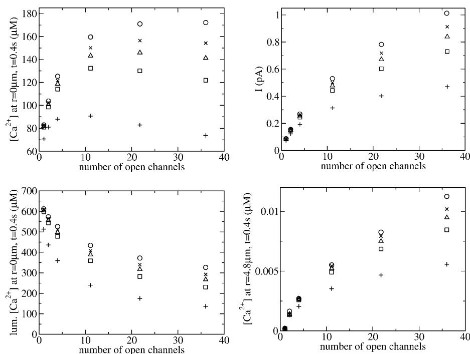
FIGURE 7 Dependence of release on the fraction of luminal mobile buffer. (Top left) Concentration of free cytosolic \text{Ca}^{2+} at the cluster in dependence on the number of open channels. (Top right) Current values. (Bottom left) Concentration of free luminal \text{Ca}^{2+} at the cluster. (Bottom right) Concentration of free cytosolic \text{Ca}^{2+} in a distance of 4.8\mu\text{m} from the cluster. (All panels) Values were taken after the channels were open for 0.4 s. In case of a single open channel in the cluster, the values were obtained after 0.115 s. For parameter values, see Set 1 in Table 1 except the concentration of luminal buffers. They are: B_{\text{Es}} = 50\text{ mM} , B_{\text{Em}} = 50\text{ mM} ( \circ ); B_{\text{Es}} = 75\text{ mM} , B_{\text{Em}} = 25\text{ mM} ( \times ); B_{\text{Es}} = 87.5\text{ mM} , B_{\text{Em}} = 12.5\text{ mM} ( \triangle ); and B_{\text{Es}} = 100\text{ mM} , B_{\text{Em}} = 0\text{ mM} ( \square ). The values marked by (+) were obtained with D_{\text{E}} = 110\mu\text{m}^2\text{s}^{-1} and B_{\text{Es}} = 100\text{ mM} , B_{\text{Em}} = 0\text{ mM} .
